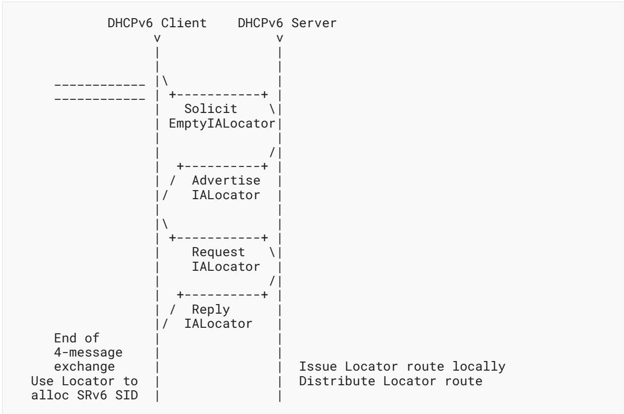
Figure 4: SRv6 Locator Exchange
