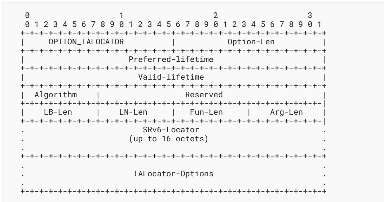
Figure 3: IA Locator Option Format
