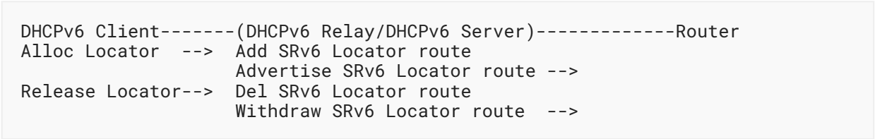
Figure 6: Advertisement of the SRv6 Locator Route
