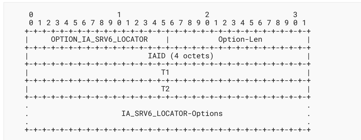
Figure 2: Identity Association for SRv6 Locator Option Format
